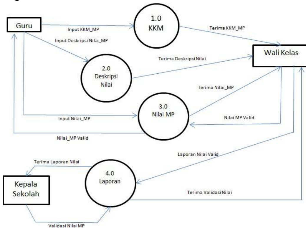
Gambar 3. Diagram nol sistem SIPK13
