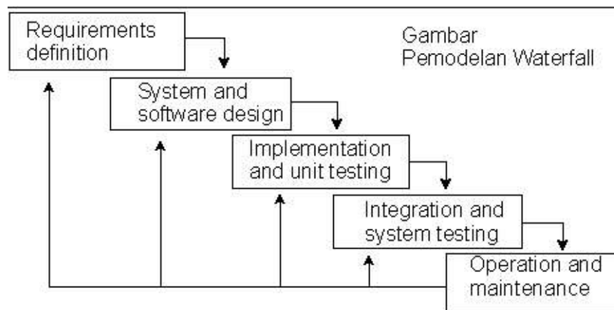
Gambar 1. Model Waterfall
