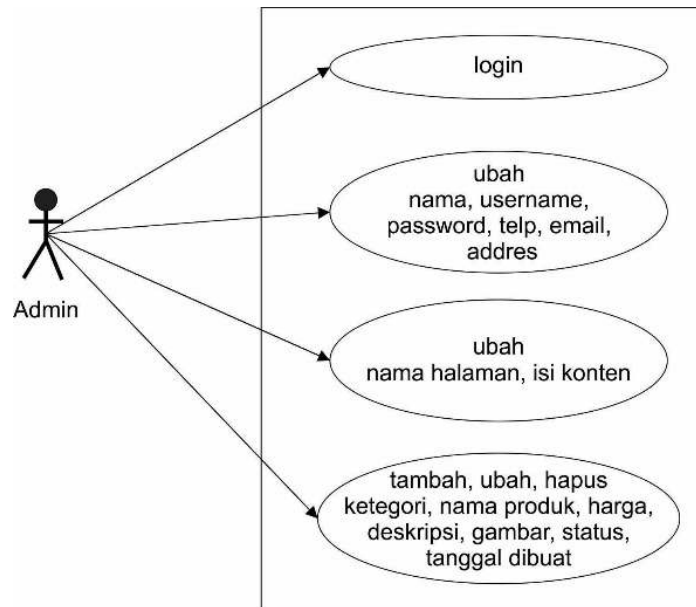
Gambar 3.2 Use Case Diagram admin website
