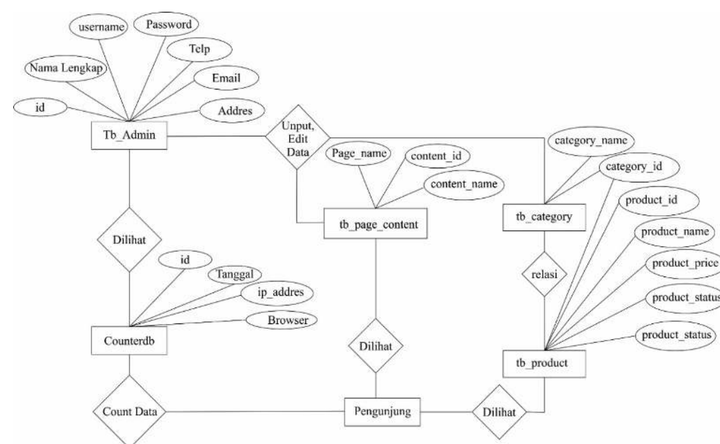
Gambar 3.8 Entity Relationship Diagram website Company Profile
